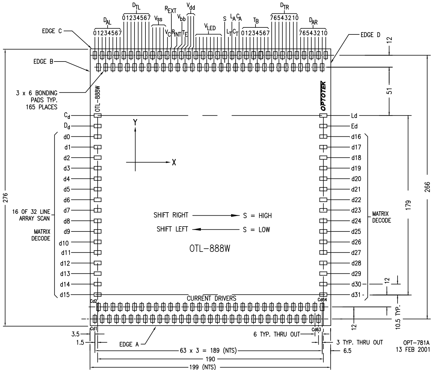
DIMENSIONS IN MILS OTL-888W CHIP SIZE AND BONDING PAD LOCATIONS Fig. 2
